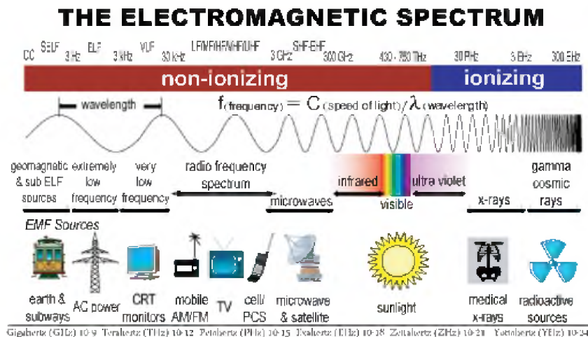
Figure 1 – Electromagnetic Spectrum (Nucleargraduates)
