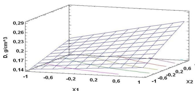
Figure 2-Response surface for density
